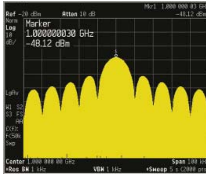
Figure 17. The PRF was set to 100 Hz (pulse period of 10 ms) pulse width of 0.1 ms, span of 100 kHz, sweep time of 5 sec and RBW of 1 kHz.
